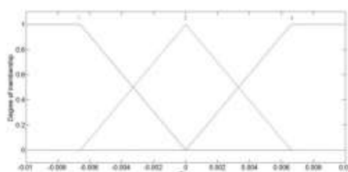
Gambar 7. Membership function delta error ( \Delta e )
