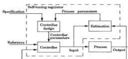
Gambar 4. Diagram bloksel f-tuning regulator
